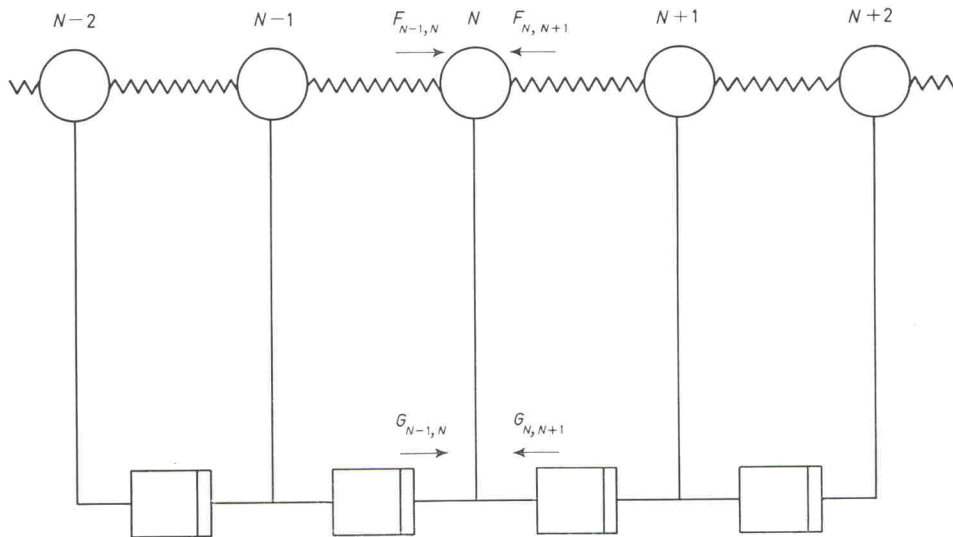
Fig. 31. - Dissipating lattice model. d^2X_N/dT^2 = F_{N-1,N} - F_{N,N+1} + G_{N-1,N} - G_{N,N+1} .
